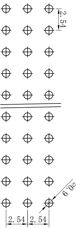
PCB LAYOUT
