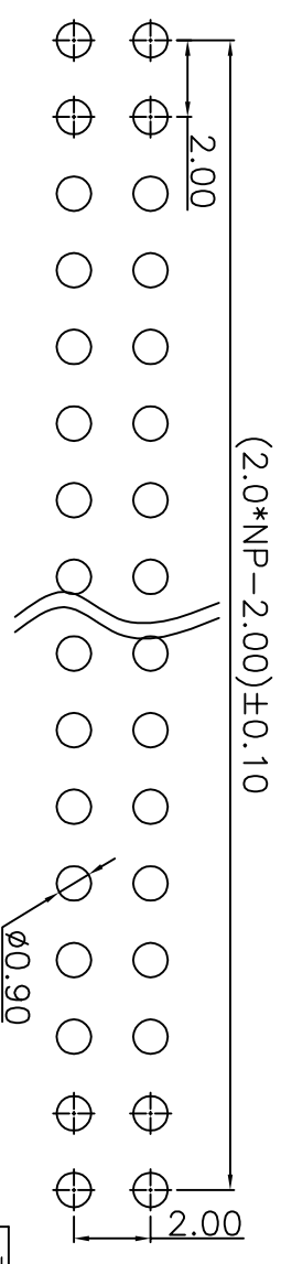
PCB LAYOUT
