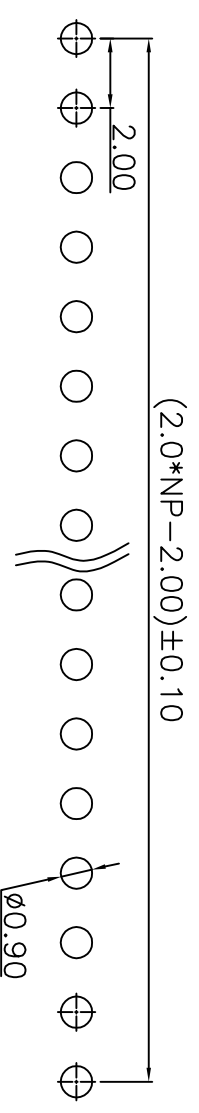
PCB LAYOUT
