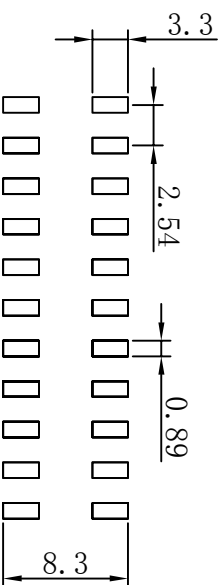
PCB LAYOUT
