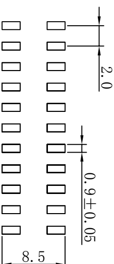
PCB LAYOUT
