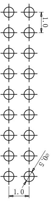
PCB LAYOUT
