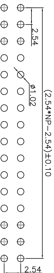
PCB LAYOUT
